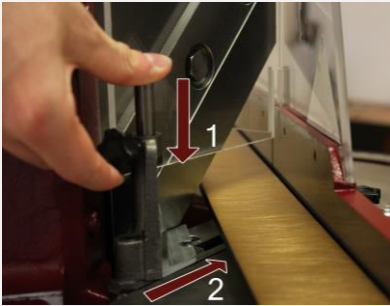
Patented spring- loaded rebate supports system
