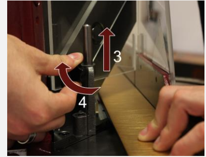
Patented spring- loaded rebate supports system
