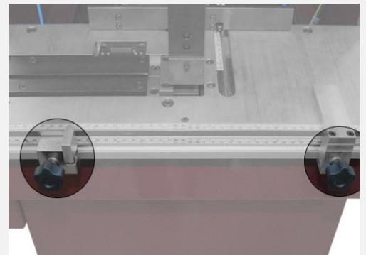
2 measure stops for setting quickly short and long sizes
