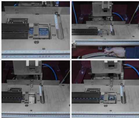
Quick switch from one hanger type tool-kit to another
